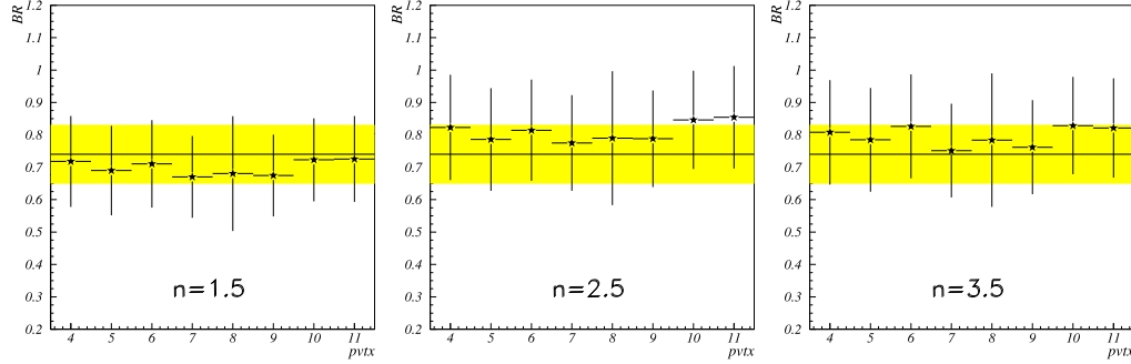
Figure 6.57: Branching ratio stability over pvtx for \frac{\Gamma(\Lambda_c^+ \rightarrow \Sigma^+ \pi^- \pi^+)}{\Gamma(\Lambda_c^+ \rightarrow p K^- \pi^+)} ; the yellow band indicates the CLEO2 measurement [4] (the most significant one performed up to now).
