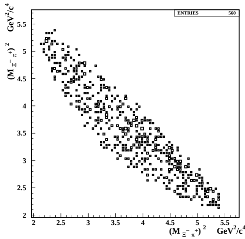
Figure 6.35: Dalitz plot for \Xi_c^+ \rightarrow \Xi^-\pi^+\pi^+ decay mode.
