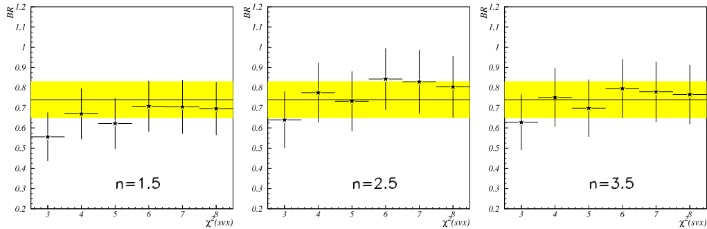
Figure 6.56: Branching ratio stability over \chi_{\text{sec}}^2 for \frac{\Gamma(\Lambda_c^+ \rightarrow \Sigma^+ \pi^- \pi^+)}{\Gamma(\Lambda_c^+ \rightarrow p K^- \pi^+)} ; the yellow band indicates the CLEO2 measurement [4] (the most significant one performed up to now).
