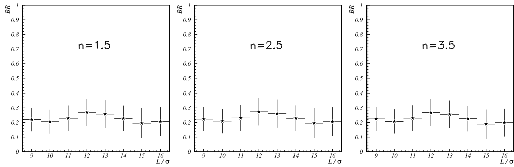
Figure 6.45: Branching ratio stability over L/\sigma for \frac{\Gamma(\Xi_c^+ \rightarrow \Sigma^- \pi^+ \pi^+)}{\Gamma(\Xi_c^+ \rightarrow \Xi^- \pi^+ \pi^+)} .
