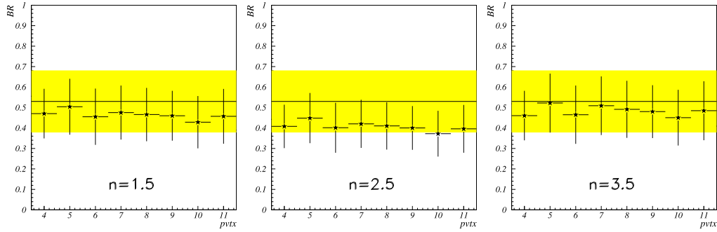
Figure 6.62: Branching ratio stability over pvtx for \frac{\Gamma(\Lambda_c^+ \rightarrow \Sigma^- \pi^+ \pi^+)}{\Gamma(\Lambda_c^+ \rightarrow \Sigma^+ \pi^- \pi^+)} ; the yellow band indicates the E687 measurement [4] (the only one performed up to now).
