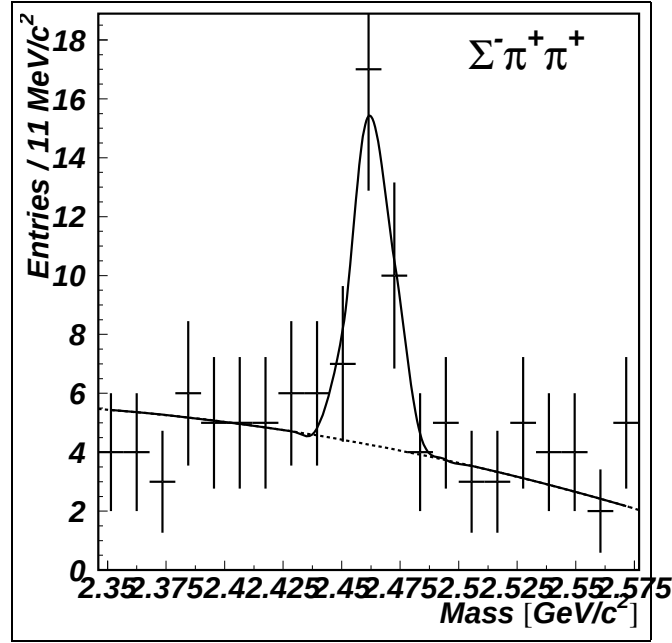
Figure 6.21: Invariant mass distribution for \Sigma^-\pi^+\pi^+ in the \Xi_c^+ mass region with \Xi_c^+ \rightarrow \Xi^-\pi^+\pi^+ reflection removed (same as Figure 6.20 but close up to the \Xi_c^+ invariant mass).
