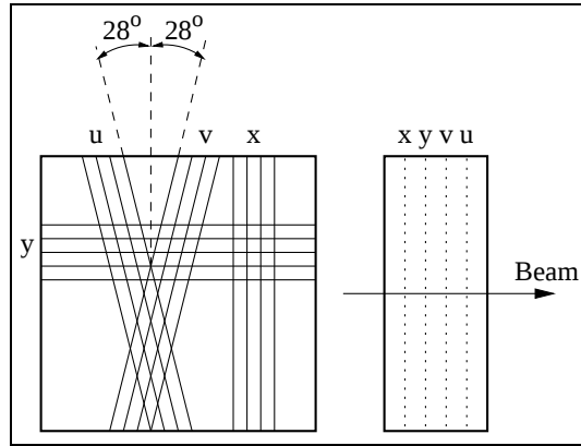
Figure 4.9: M1 chamber.
