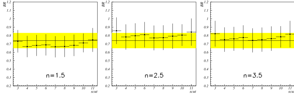
Figure 6.58: Branching ratio stability over scut for \frac{\Gamma(\Lambda_c^+ \rightarrow \Sigma^+ \pi^- \pi^+)}{\Gamma(\Lambda_c^+ \rightarrow p K^- \pi^+)} ; the yellow band indicates the CLEO2 measurement [4] (the most significant one performed up to now).
