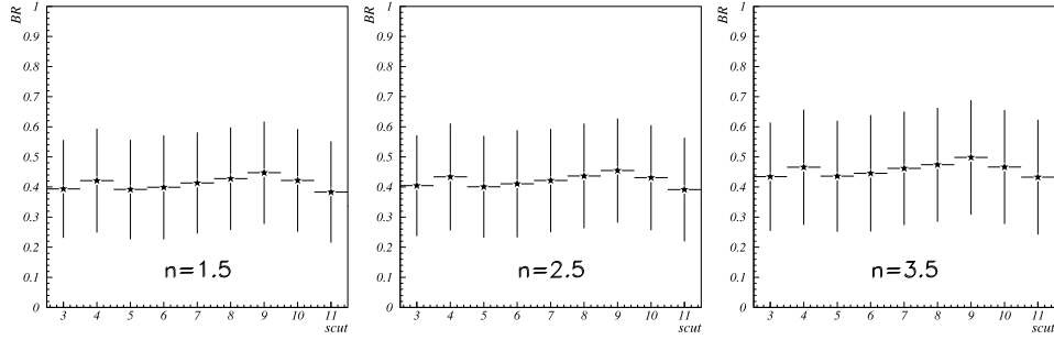
Figure 6.43: Branching ratio stability over scut for \frac{\Gamma(\Xi_c^+ \rightarrow \Sigma^+ \pi^- \pi^+)}{\Gamma(\Xi_c^+ \rightarrow \Xi^- \pi^+ \pi^+)} .
