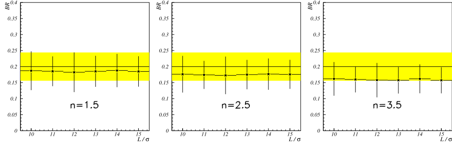
Figure 6.50: Branching ratio stability over L/\sigma for \frac{\Gamma(\Xi_c^+ \rightarrow pK^- \pi^+)}{\Gamma(\Xi_c^+ \rightarrow \Xi^- \pi^+ \pi^+)} ; the yellow band indicates the previous SELEX measurement [7].
