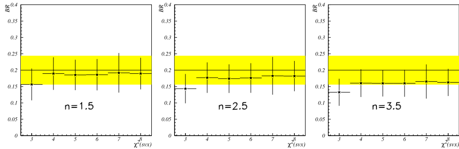
Figure 6.51: Branching ratio stability over \chi_{\text{sec}}^2 for \frac{\Gamma(\Xi_c^+ \rightarrow pK^- \pi^+)}{\Gamma(\Xi_c^+ \rightarrow \Xi^- \pi^+ \pi^+)} ; the yellow band indicates the previous SELEX measurement [7].
