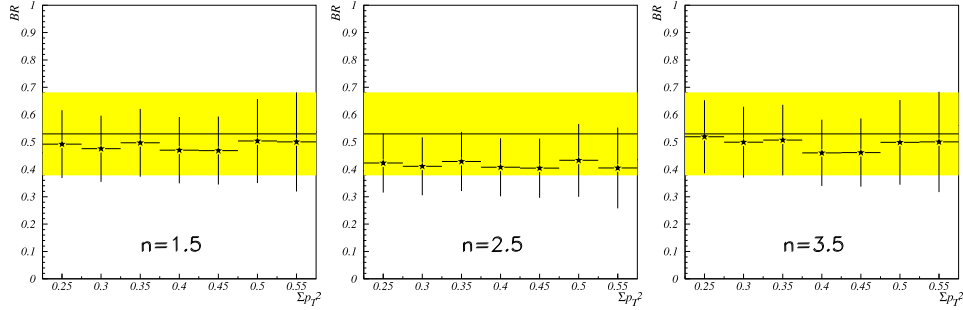
Figure 6.64: Branching ratio stability over p_T^2 for \frac{\Gamma(\Lambda_c^+ \rightarrow \Sigma^- \pi^+ \pi^+)}{\Gamma(\Lambda_c^+ \rightarrow \Sigma^+ \pi^- \pi^+)} ; the yellow band indicates the E687 measurement [4] (the only one performed up to now).
