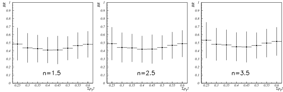
Figure 6.44: Branching ratio stability over p_T^2 for \frac{\Gamma(\Xi_c^+ \rightarrow \Sigma^+ \pi^- \pi^+)}{\Gamma(\Xi_c^+ \rightarrow \Xi^- \pi^+ \pi^+)} .
