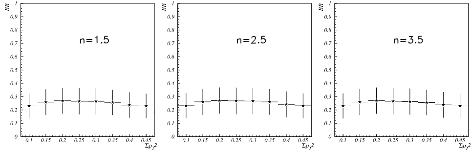
Figure 6.49: Branching ratio stability over p_T^2 for \frac{\Gamma(\Xi_c^+ \rightarrow \Sigma^- \pi^+ \pi^+)}{\Gamma(\Xi_c^+ \rightarrow \Xi^- \pi^+ \pi^+)} .
