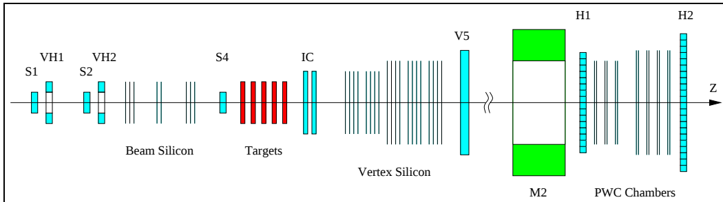
Figure 4.15: SELEX trigger.
