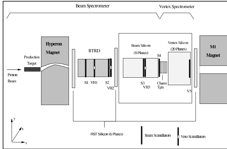
Figure 4.4: Schematic view of the beam spectrometer.
